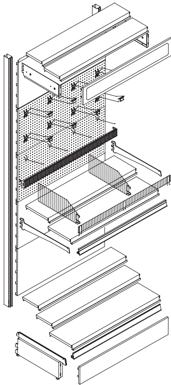
Elementi a parete con piani a liste, piani interi e accessori Wall units with plank shelves, one piece shelves and accessories
