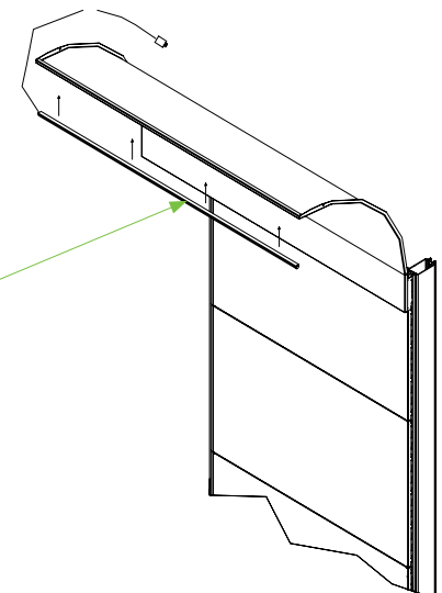
Cielino vela curvo h 55 cm Circular canopy h 55 cm
