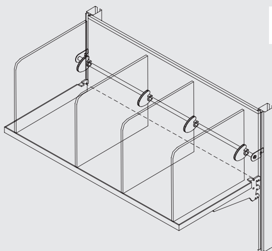
Barra reggi morsetti su piano in legno Pigeonholes with clamps on wooden shelf
