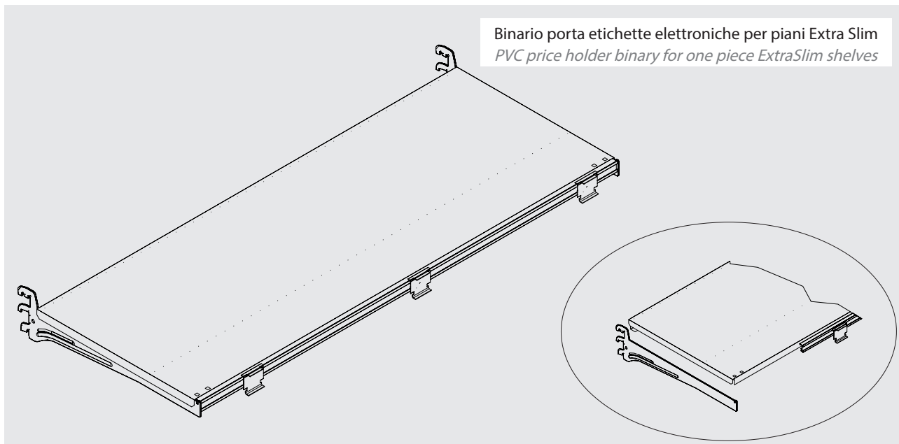
Binario biestruso PVC portaetichette per piani Extra Slim PVC price holder binary for one piece ExtraSlim shelves
