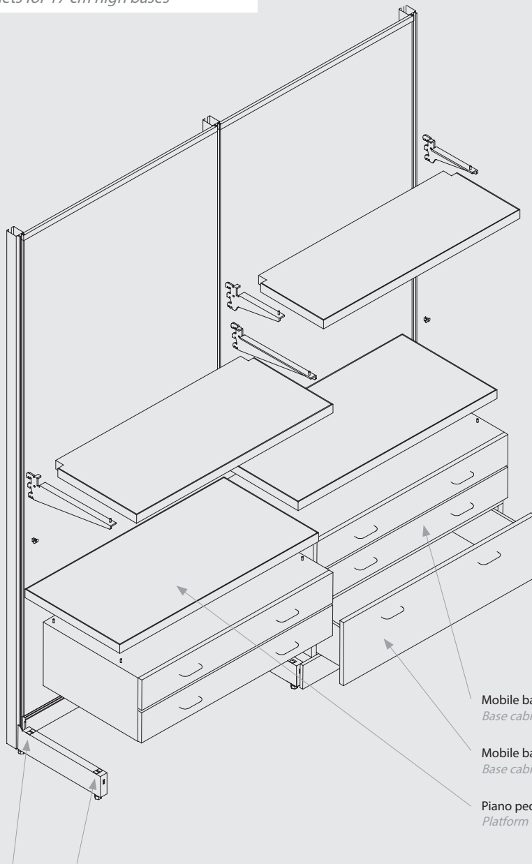
Supporti per piano pedana: 2.9 Supports for platform top: 2.9
