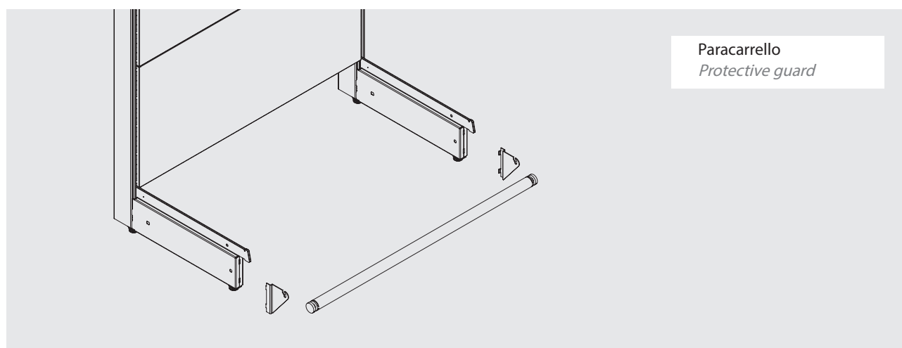
Traverso paracarrello Crosspiece for protective guard
